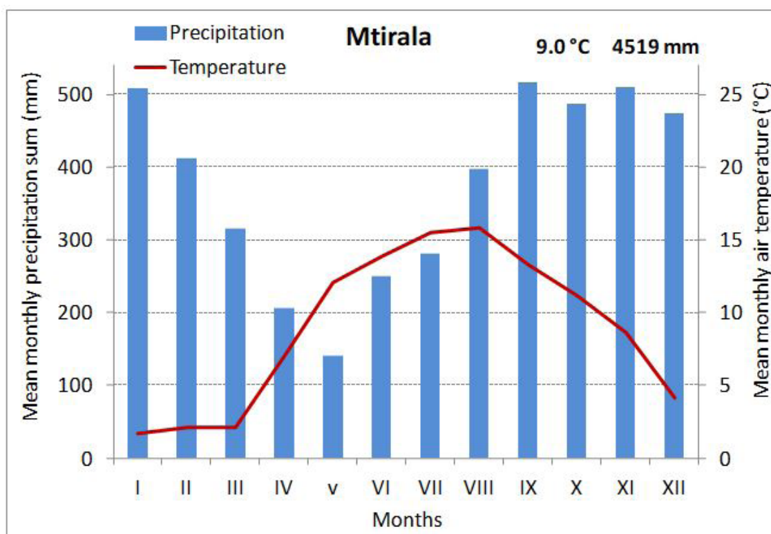
Figure 43. Climate diagram of Mount Mtirala, Mtirala-Kintrishi nominated component area. Source: Mtirala climate station data 1980 – 85.
